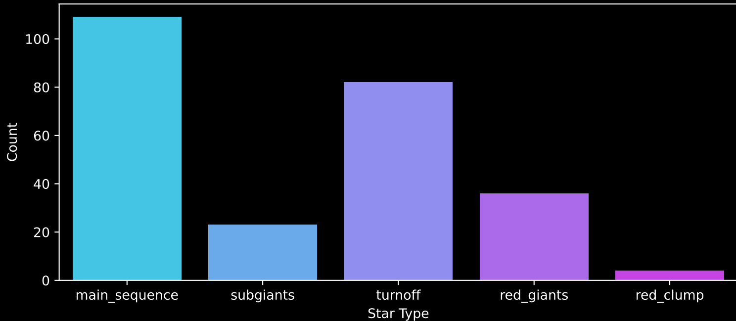
GALAH DR4 Field: [1857] Count plot of Star Type
