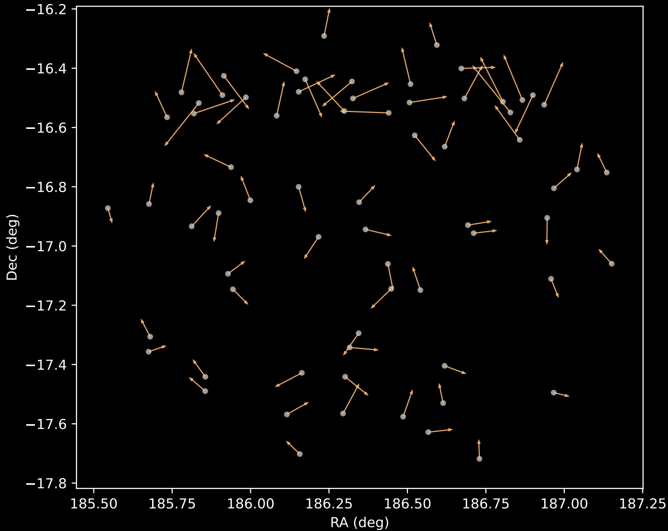
GALAH DR4 Cluster 3 Proper Motion Vectors (n=69)
