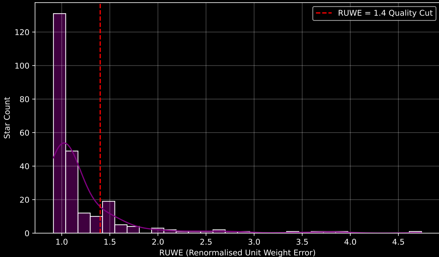
GALAH DR4 Field [1857] RUWE Distribution (n= 247)
